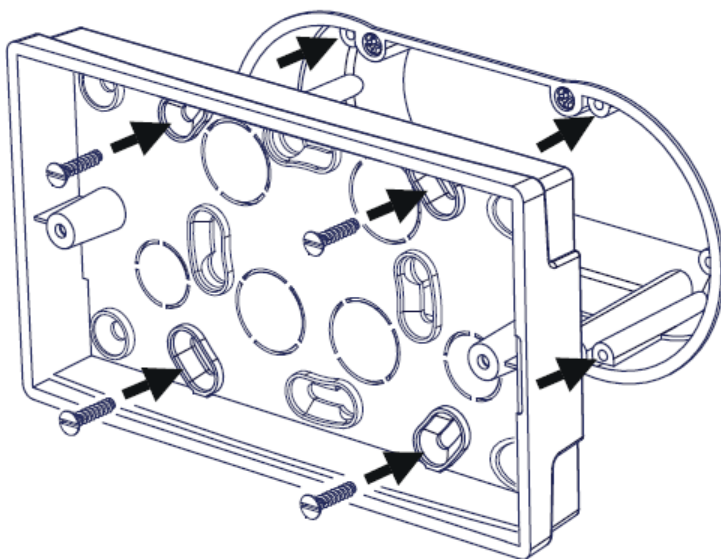
71mm x 60mm Euro back box
